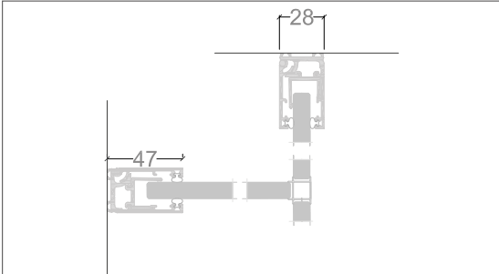
"T" JUNCTION
