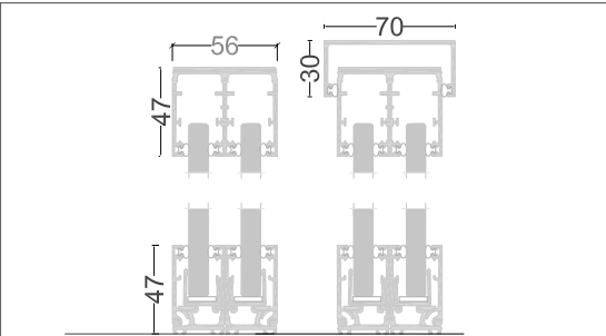
VERTICAL SECTION
