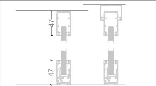
VERTICAL SECTION
